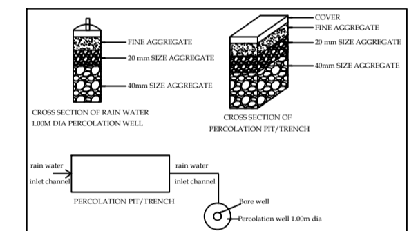
DETAILS OF RAIN WATER HARVESTING STRUCTURES
