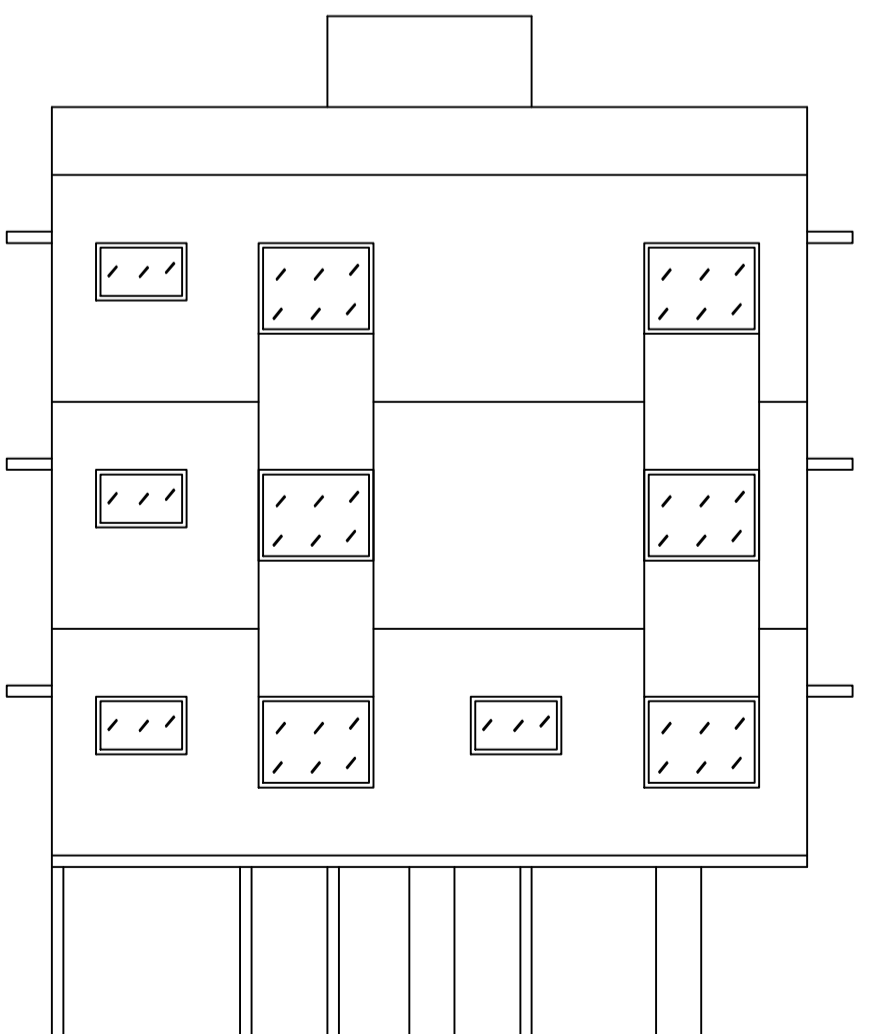
FRONT ELEVATION
